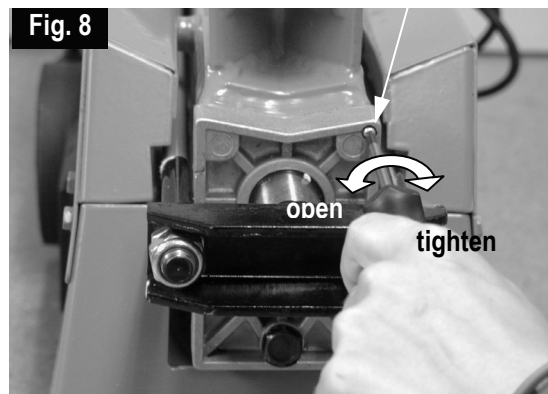
Bleed screw
